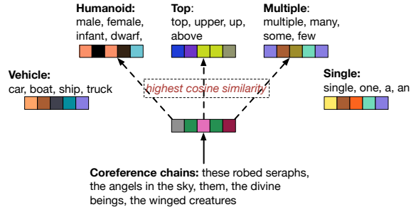
Figure 2: Using word2vec representations from coreferent groupings in a description to deduce object class and attributes by cosine similarity.
